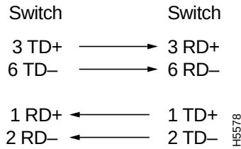
Figure B-5 Straight-Through Cable Pinouts
