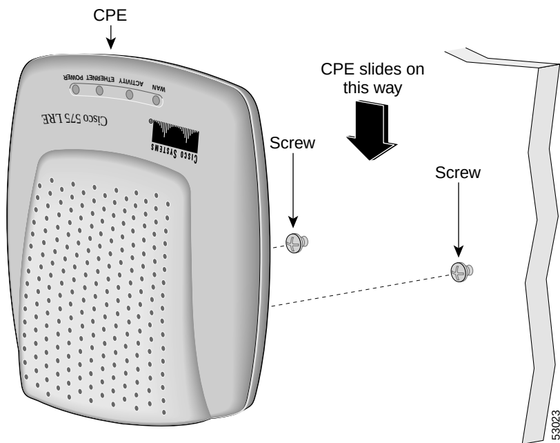
Figure 2-4 Installing the CPE On a Wall
