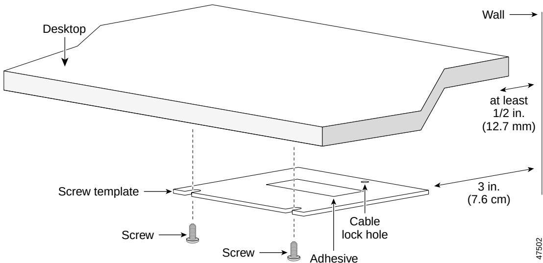
Figure 2-1 Installing the Mounting Screws Under a Desk
