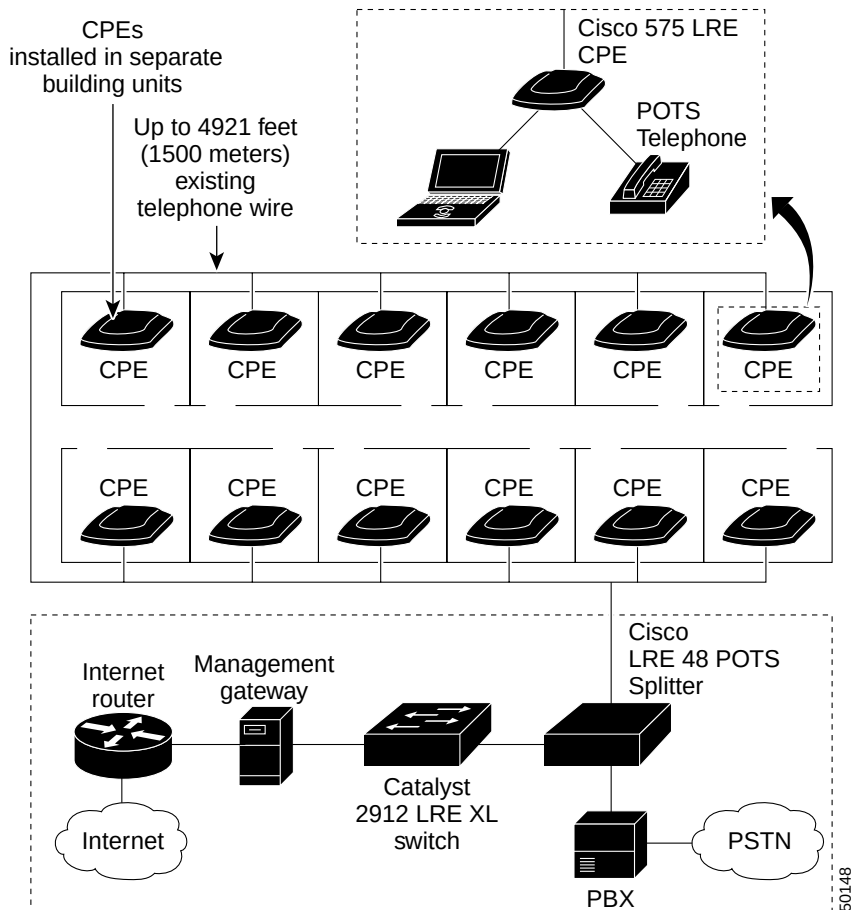
Figure 1-1 Typical LRE Installation
