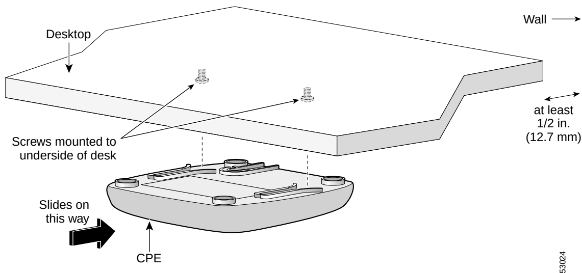
Figure 2-2 Mounting the CPE Under a Desk
