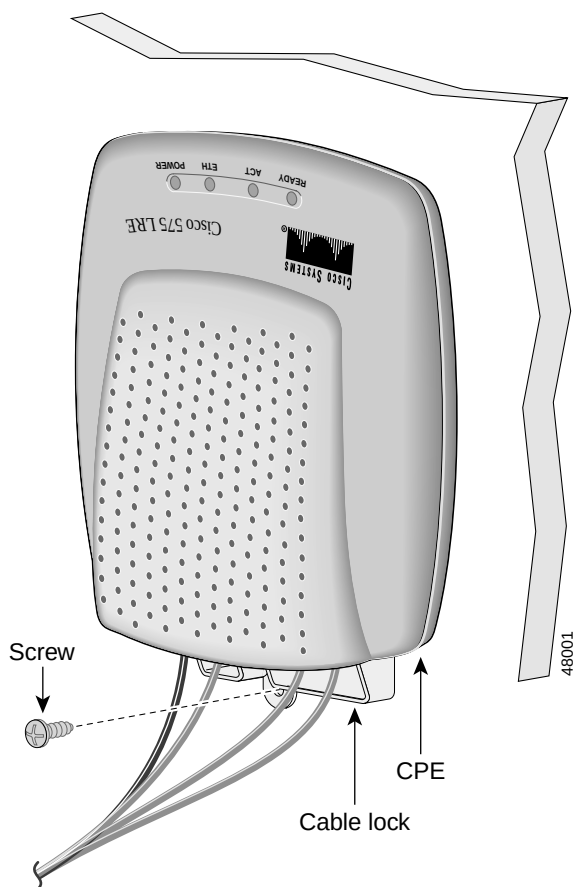
Figure 2-11 Securing the Cable Lock with Mounting Screw
