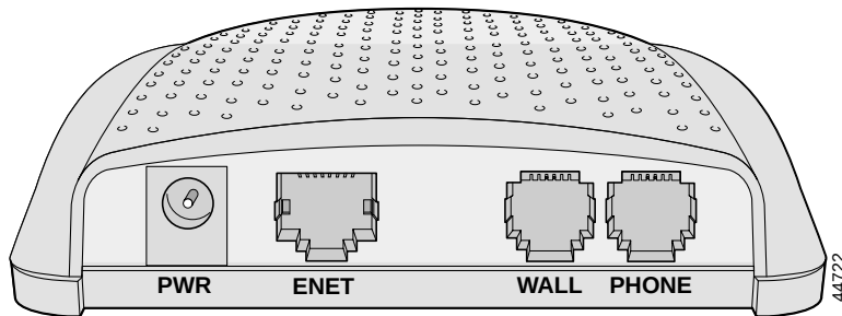
Figure B-1 CPE Connectors
